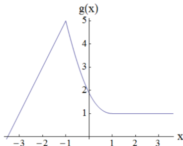
The graph of a function y = g(x)
