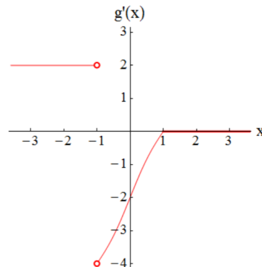
The graph of the derivative y = g'(x)
